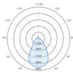
70° Reflector
