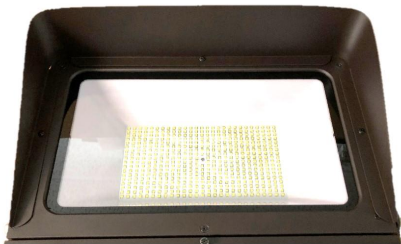
Glare shield mounted on a UFB fixture
