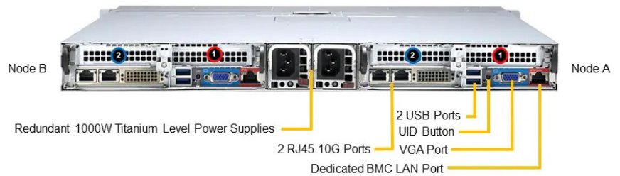
SM3-1204 Rear View—System
